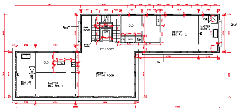
SECOND FLOOR PLAN 2樓平面圖
