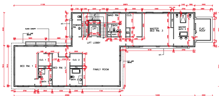
FIRST FLOOR PLAN 1樓平面圖
