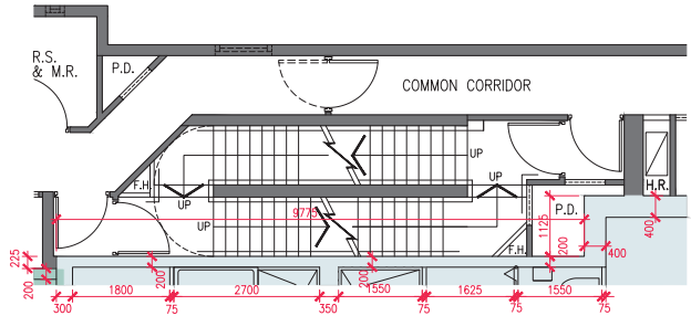
PART PLAN AT 29/F 29樓 局部平面圖
