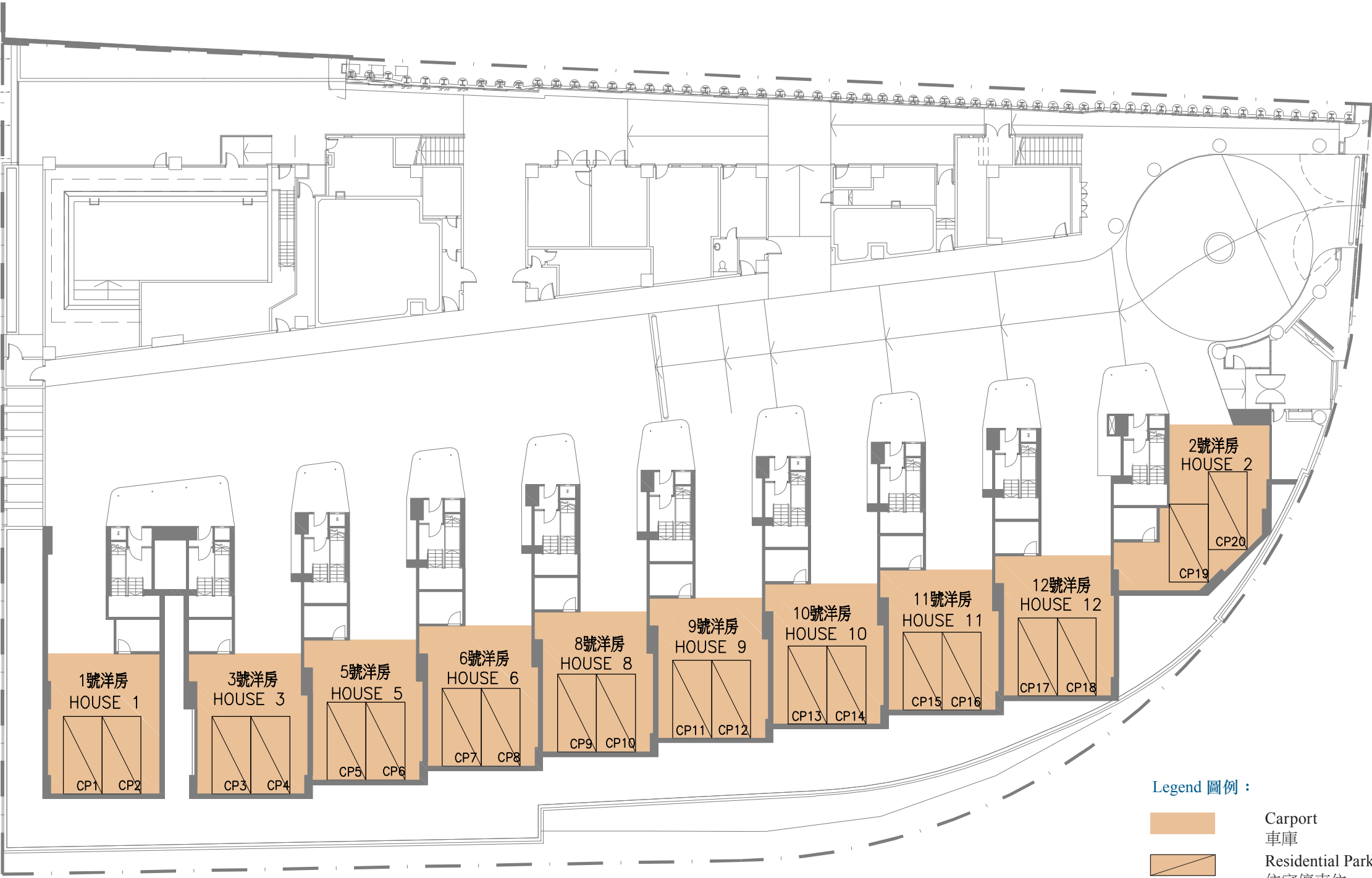
Lower Ground Floor Plan 低層地下平面圖
