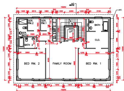
FIRST FLOOR PLAN 1樓平面圖
