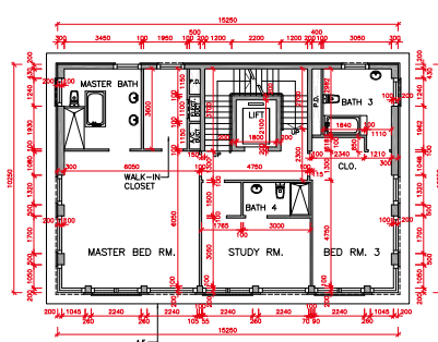
SECOND FLOOR PLAN 2樓平面圖
