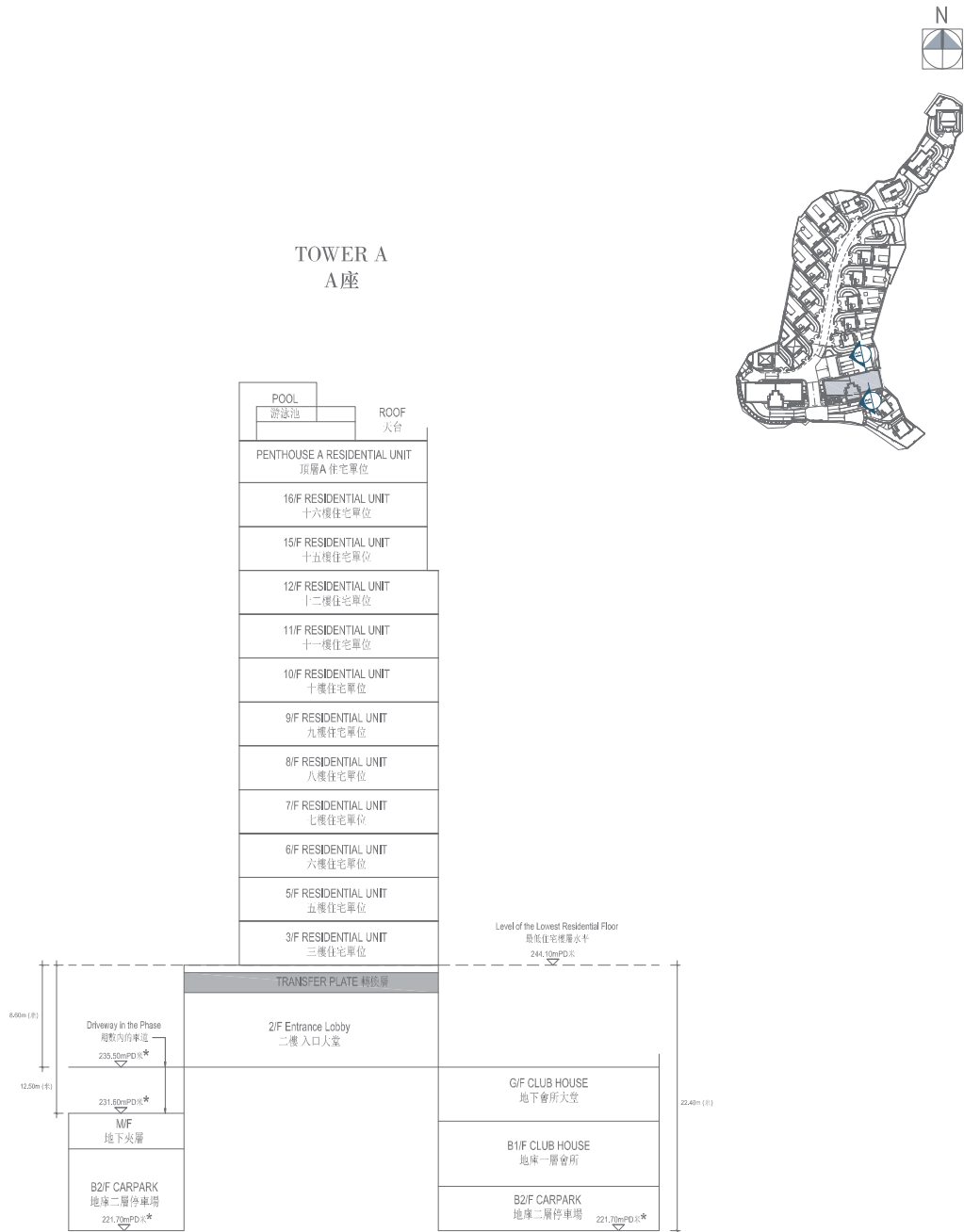
Section B 剖面圖B
