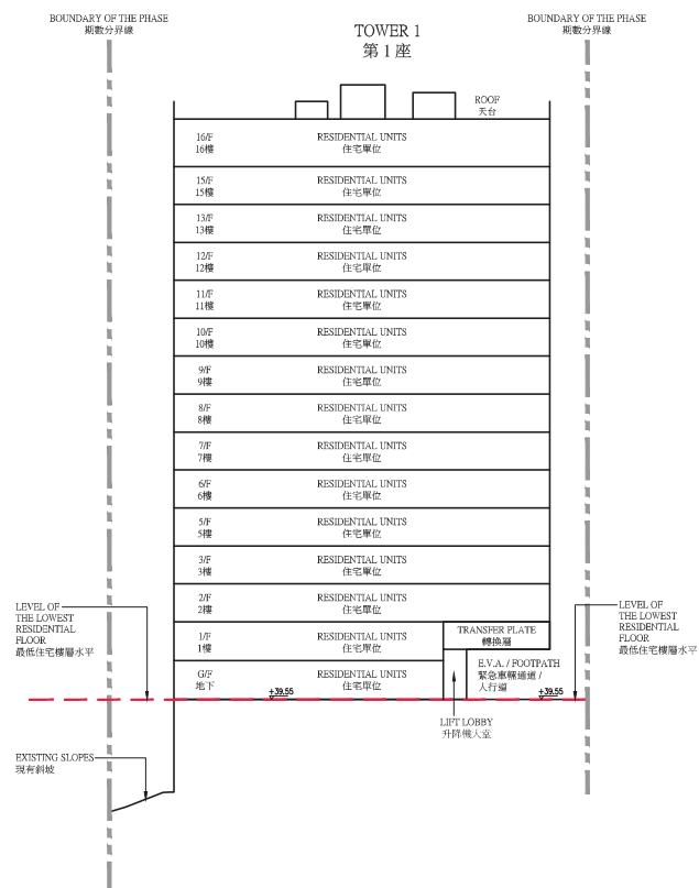
CROSS-SECTION PLAN B-B 橫截面圖B-B
