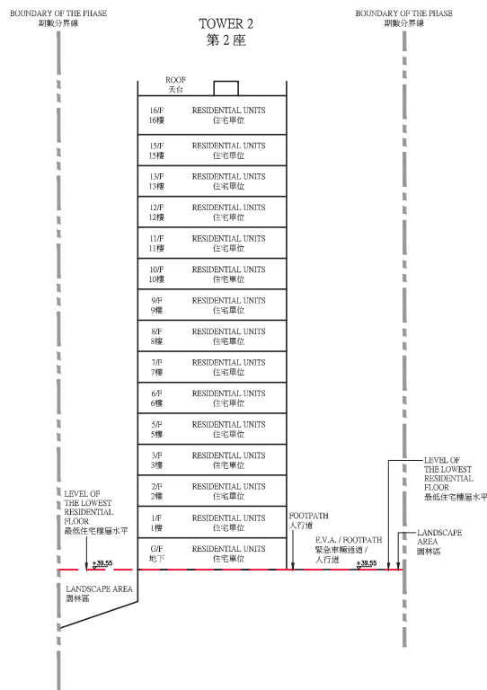
CROSS-SECTION PLAN C-C 橫截面圖C-C
