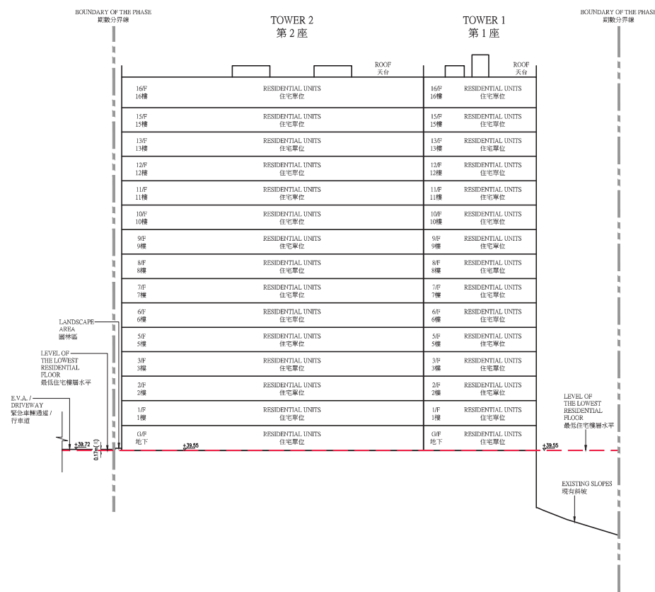
CROSS-SECTION PLAN A-A 橫截面圖A-A
