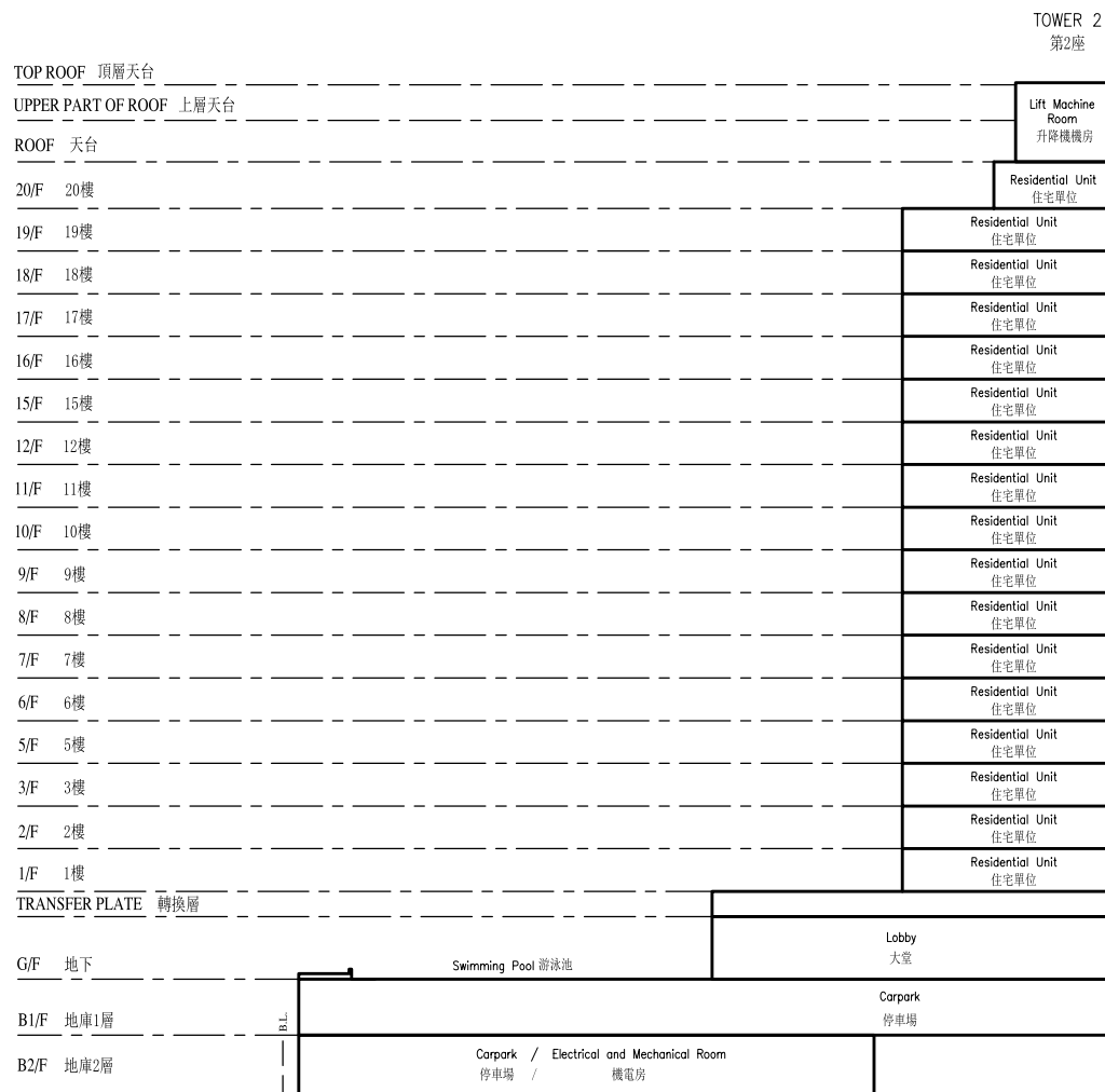
CROSS SECTION PLAN A - A 橫截面圖 A - A
