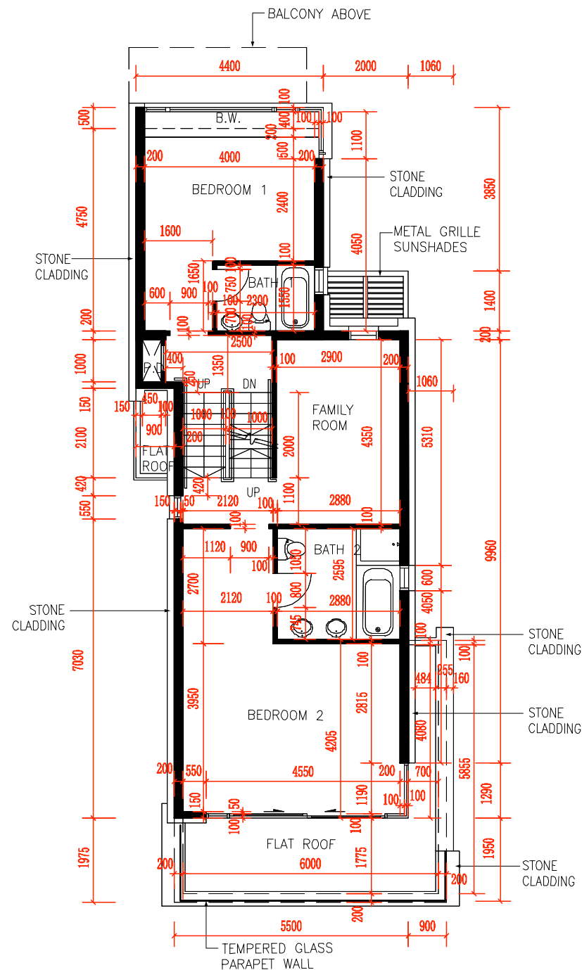
FIRST FLOOR PLAN (1/F PLAN)
