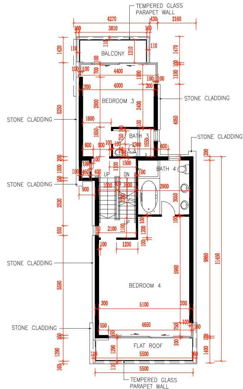
SECOND FLOOR PLAN (2/F PLAN)
