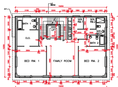
FIRST FLOOR PLAN 1樓平面圖
