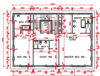
SECOND FLOOR PLAN 2樓平面圖
