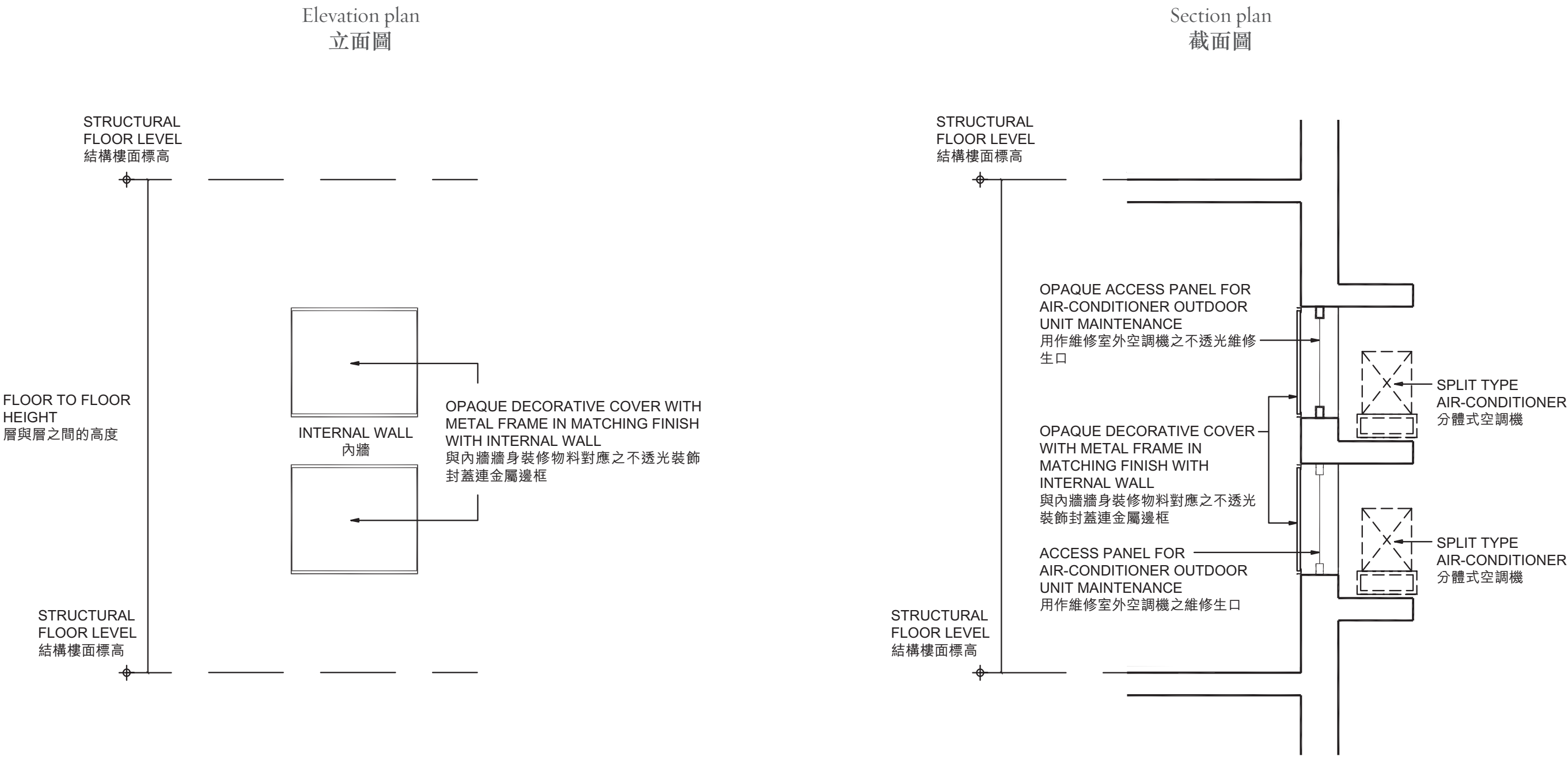
Brief elevation plan and section plan of removable decorative cover, access panel and air-conditioner hood at high level and low level 可拆除的裝飾封蓋、維修生口及空調機遮簷設於高位及低位之簡要立面圖和截面圖
