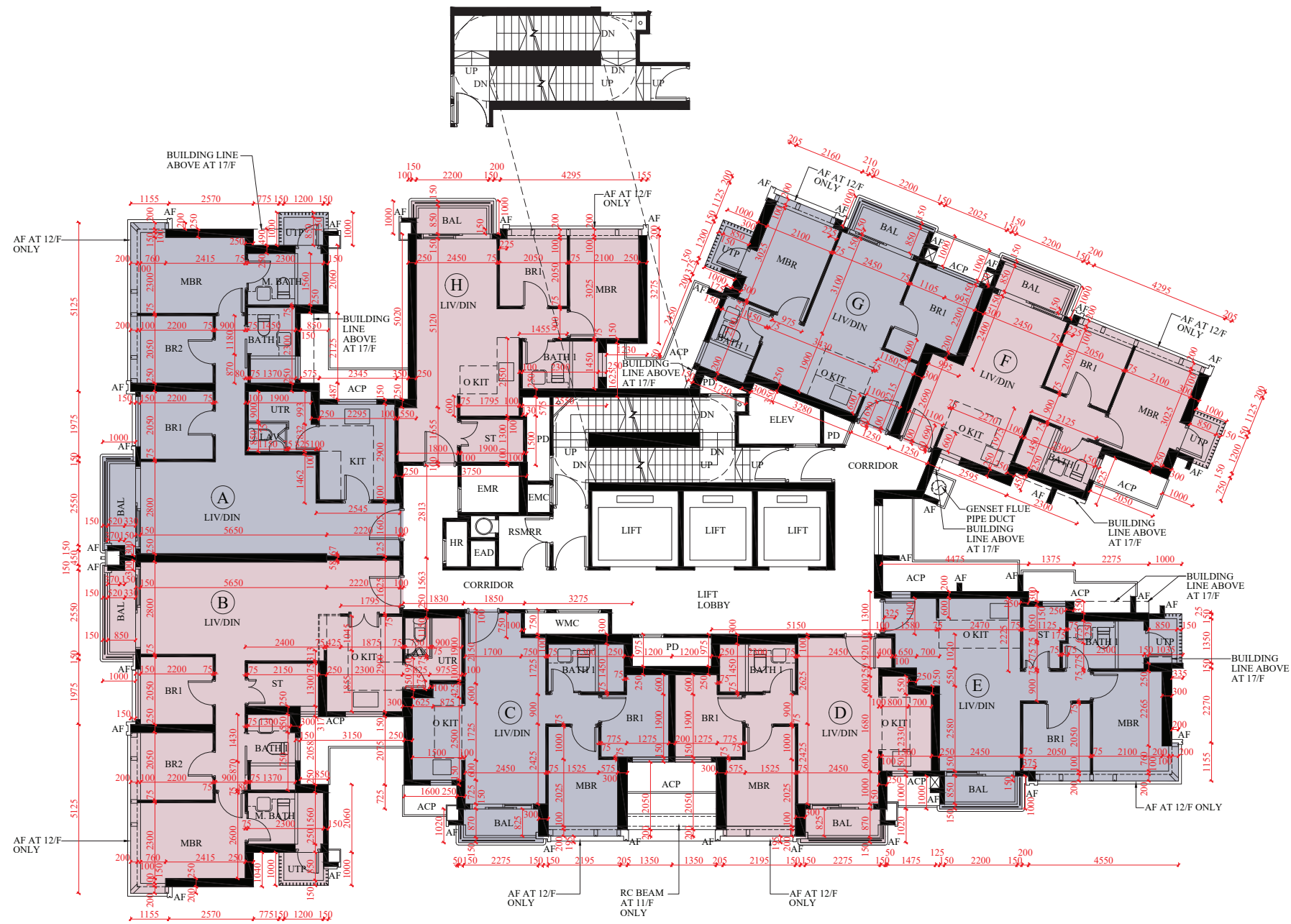
PART PLAN OF 16/F 16樓部分平面圖
