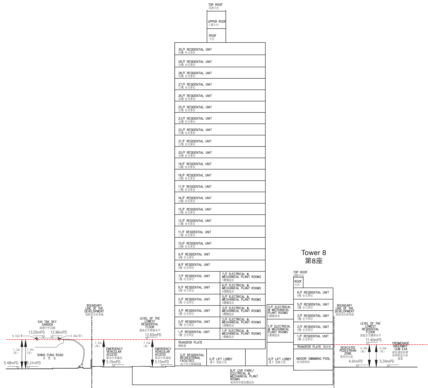
Cross-section Plan G-G 橫截面圖G-G
