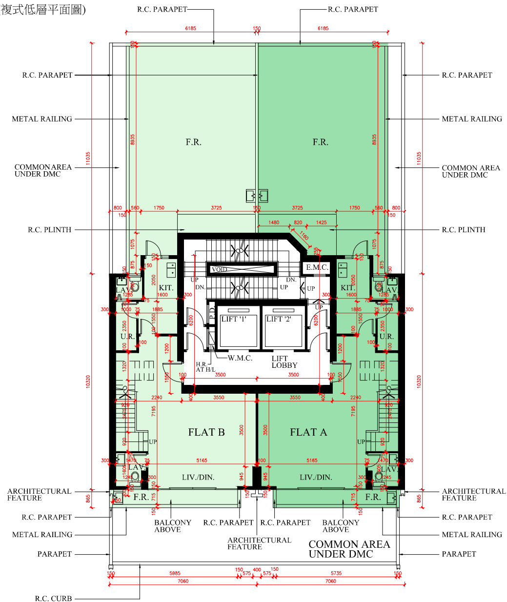
2/F FLOOR PLAN (LOWER DUPLEX FLOOR PLAN)
